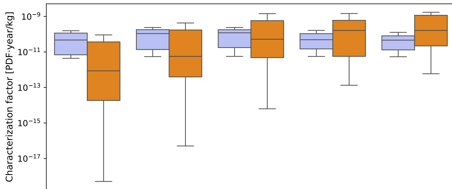
GLAM
